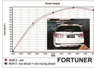
The test of Eco Diesel + Biodiesel on Toyota Fortuner showed the power and torque increase surpassing the pure Biodiesel
